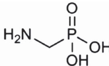
aminomethylphosphonic acid
